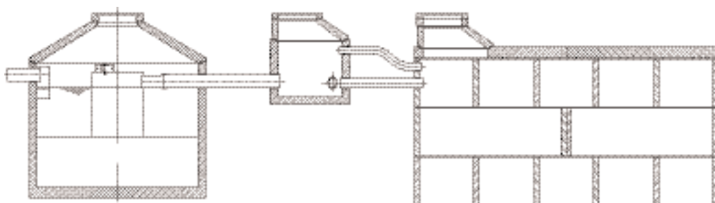
Mall-Sedimentationsanlage
